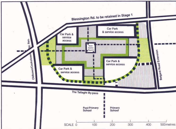
DRAWING D Structure map – the first stages
