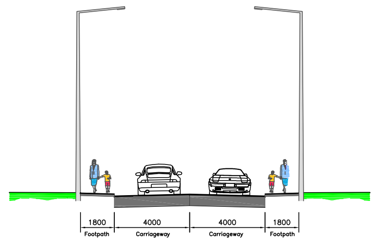
SECTION A 1:100
