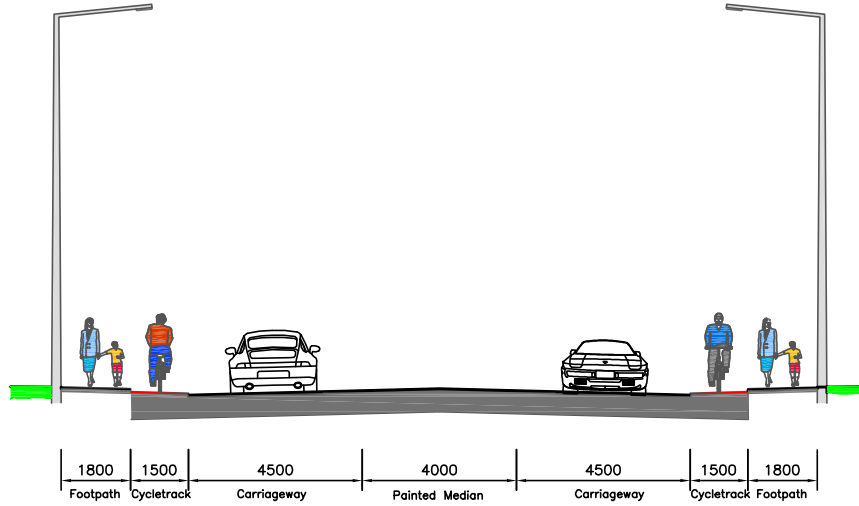
SECTION B 1:100
