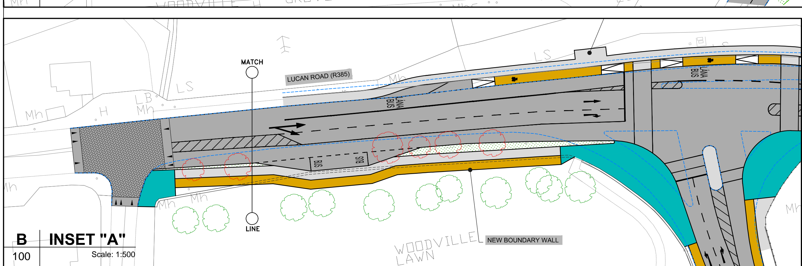
A GENERAL ARRANGEMENT Scale: 1:500
